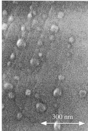
Fig.5 SEM image of 3C-SiC epilayer surface by APCVD. Flow rate of \text{SiH}_4 : 0.8 sccm, \text{C}_3\text{H}_8 : 0.6 sccm and \text{H}_2 : 8 slm.
