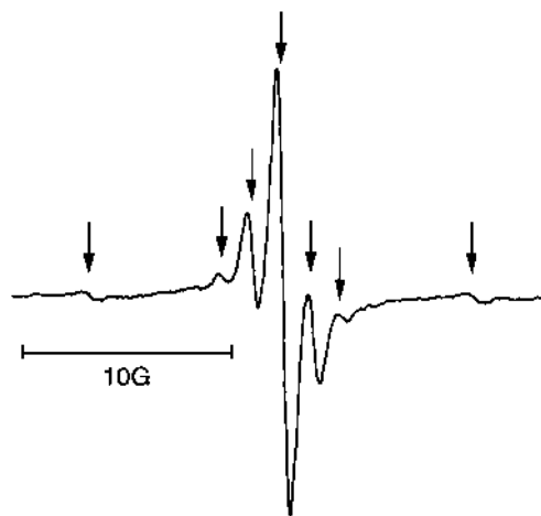
Fig.3 ESR spectrum at room temperature for 3C-SiC irradiated with electrons at 3 \times 10^{18} / \text{cm}^2 . The magnetic field was applied parallel to the \langle 100 \rangle axis. ESR lines of the T1 signal, which arises from a negatively charged silicon vacancy, are indicated by the arrows.
