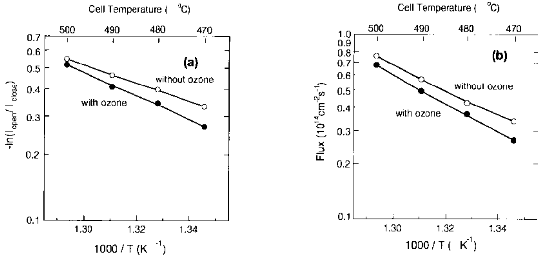
Fig. 5 (a) AAS signal (-\ln(I_{open}/I_{close})) for Sr, and (b) Sr flux rate determined by ICP as a function of the effusion-cell temperature. Introducing ozone shows reductions of Sr flux and AAS signal.
