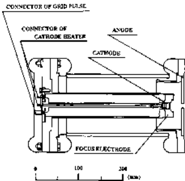
Fig.6 Cross-sectional drawing of the electron gun.
