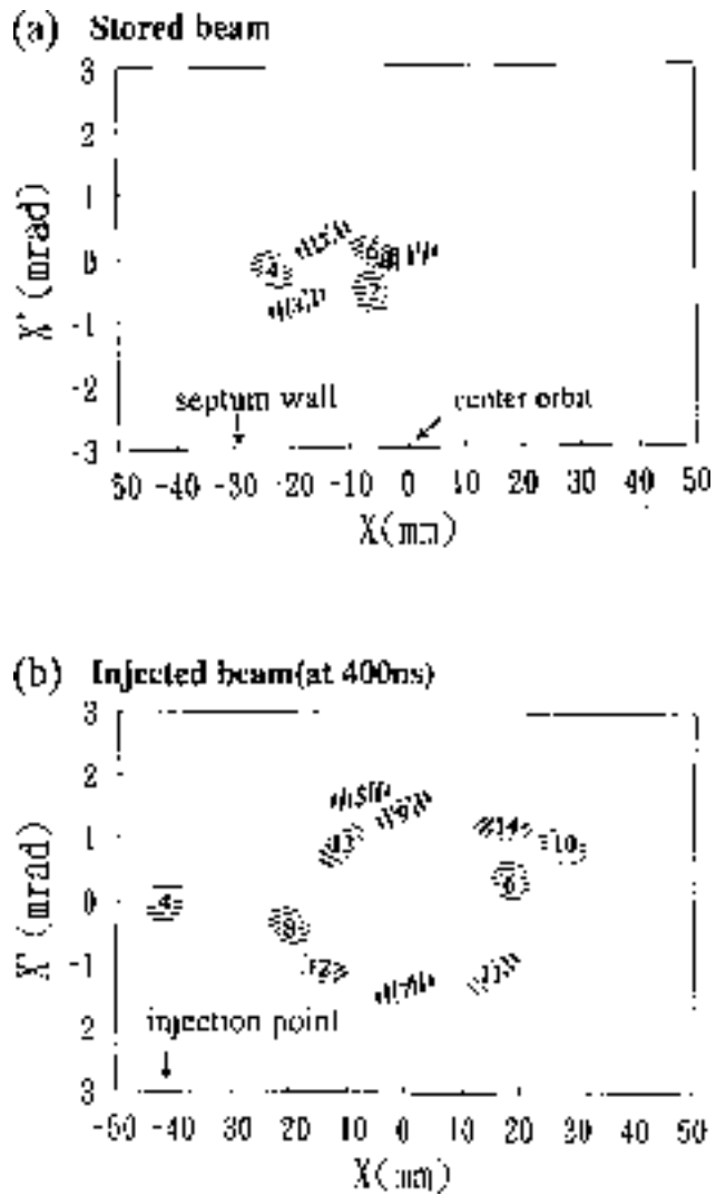
Fig.3 The beam tracking results of (a) the stored beam and (b) the injection beam at 400 ns of the kicker magnet excitation. Indicated numbers 1, 2, ... denote the number of turns. The ellipses are phase space of electrons. The electron beam is injected at 400 ns of the kicker magnet excitation. So the first turn number of the injection beam is the fourth of the stored beams. The orbit of the stored beam is distorted to the septum wall by the excited kicker magnet during third to fifth turns and at that time the injection beam is able to be stored in the ring. All the injection electrons at 40 ns of the kicker excitation can circulate 12 turns without colliding with the septum wall and the storage rate is 1.0.
