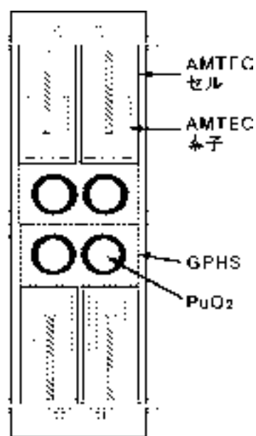
Fig.3 OSC AMTEC generator design
