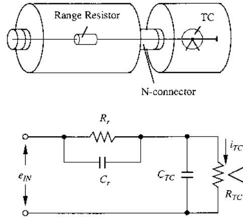
Figure 6.7 The equivalent circuit diagram of the TC-Range resistor combination. The capacitance C_{TC} shunts the heater resistance R_{TC} and C_r shunts the current-limiting resistor R_r .
